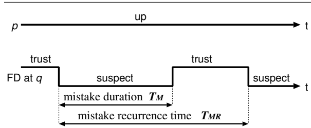
Figure 4. Quality of service metrics describing wrong suspicions made by failure detectors. Process q monitors process p .
