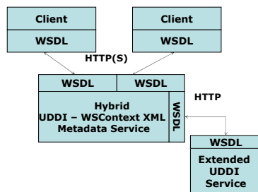
Figure 1. This figure illustrates the two clients interacting with the Hybrid UDDI – WSContext XML Metadata Service, while the hybrid service is interacting with an external UDDI Service for handling and discovering of static metadata.
