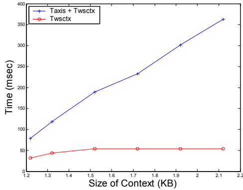
Figure 3. Comparison between (T_{axis} + T_{wscctx}) and T_{wscctx}
