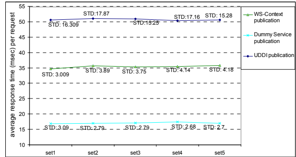
Figure 2. Average Response Time Graph for Publication Requests.
