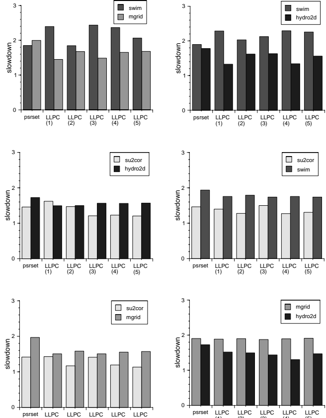
Figure 2. Comparing the slowdown factors of LLPC to the Solaris processor set ( psrset ) static partitioning mechanism when executing two parallel applications simultaneously. Five different runs of the LLPC-enabled applications are shown to demonstrate its potential variability.
