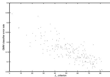
Figure 2. Scatter plot of GMM classifier EER and J_\omega value for size 12 subsets ( \rho = -0.79 )
