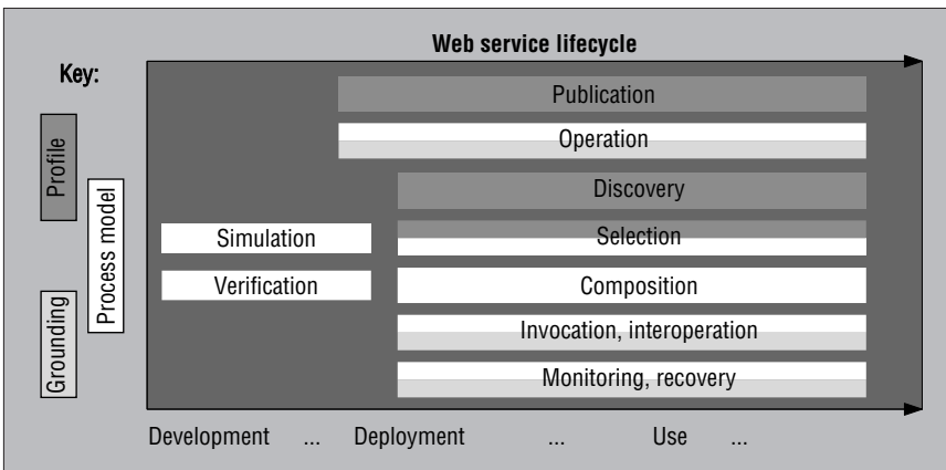
Figure 2. Applicability of the DAML-S profile, process model, and grounding ontologies to activities within the Web service lifecycle.
