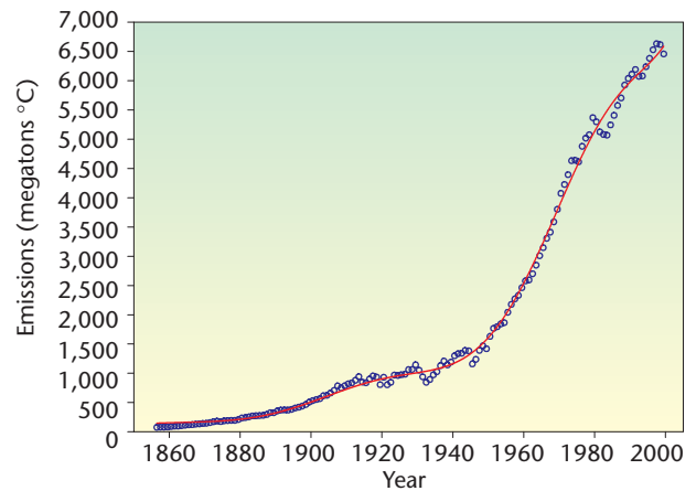
Figure 3. Nonlinear fit of the exponential–sinusoidal model in Equation 6 to the global total fossil fuel emissions for the years 1856 through 1999.
