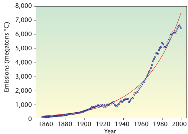
Figure 1. The nonlinear fit of the simple exponential model in Equation 1 to the global total fossil fuel emissions for the years 1856 through 1999.
