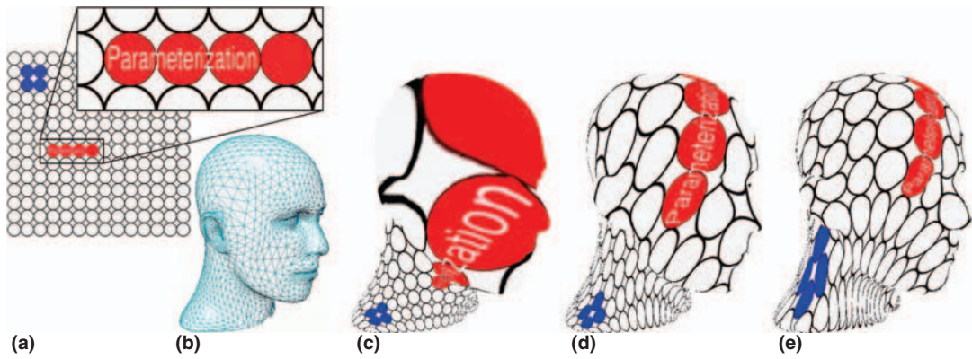
Figure 1: Texture mapping of the Mannequin Head model with three mesh parameterizations used in our method. (a) Texture and model. (b) Floater's shape preserving parameterization [6] is used as an initial mesh parameterization. (c) After a single optimization pass. (d) Our optimal low-stretch parameterization.
