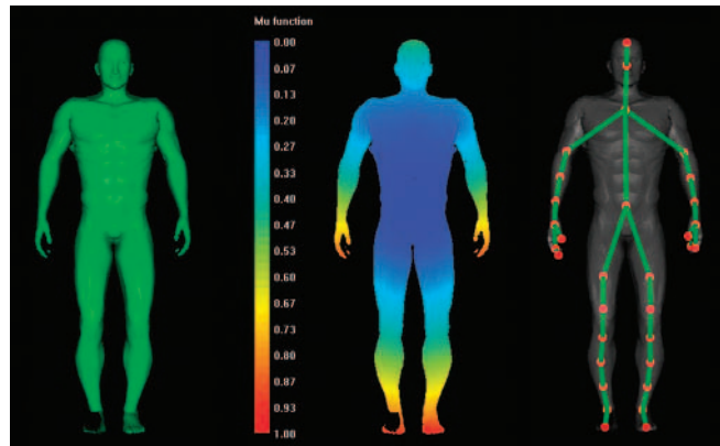
Figure 2. Reeb graph: 3D model (left), function \mu N (middle), Reeb graph; edges in green; nodes in red (model from [23]).
