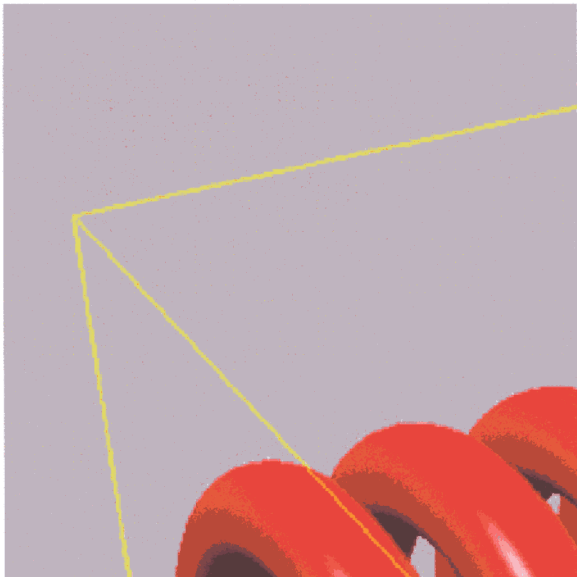
Figure 1: Example of a torus replication
