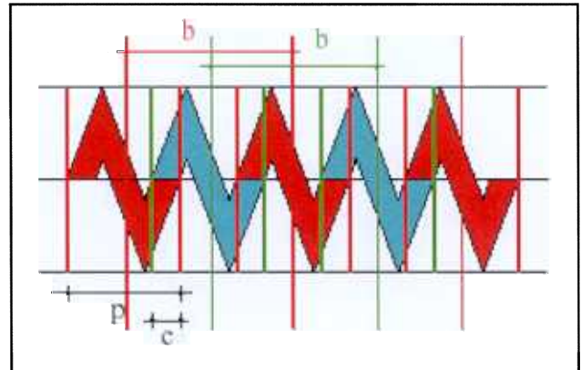
Figure 2: Overlapping of replicated regions
