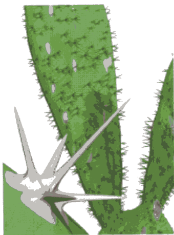
Color plate 2: A cactus generated by alternating between growing and subdivision steps.
