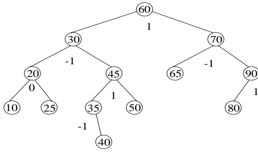
Figure 3. An example of AVL tree.
