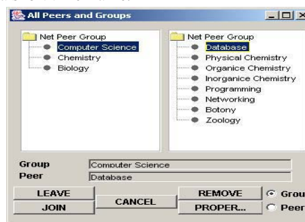
Figure: Interface to "Community Builder" in JXTA
