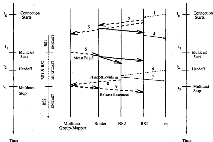
Figure 4: Protocol and Message Flow
