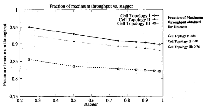
Figure 6: Avg. Throughput vs stagger
