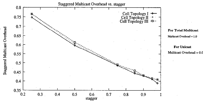
Figure 7: Avg. Multicast Overhead vs stagger
