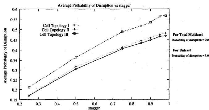
Figure 5: Avg. Prob. of Disruption vs stagger
