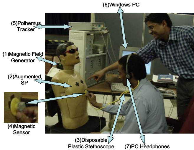
Figure 1. Prototype System
