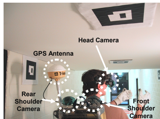
Figure 1 – Hardware configuration with three video cameras, GPS antenna, and fiducial markers on the hands and building
