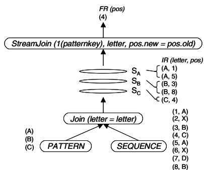
Figure 5: QEP for the usage of the StreamJoin operator in pattern recognition.
