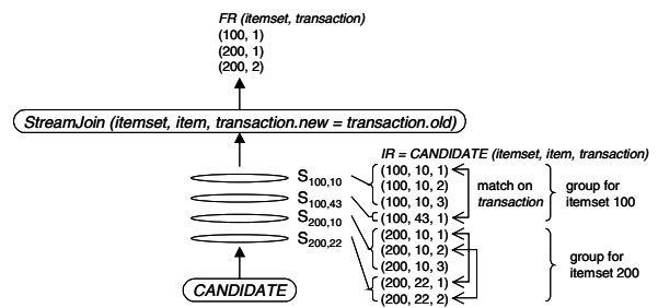
Figure 1: StreamJoin processing for an input stream of candidate itemsets.
