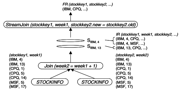
Figure 4: QEP for the usage of the StreamJoin operator in financial time series.
