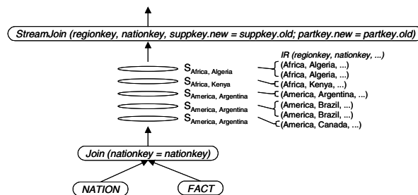
Figure 3: Simplified QEP for an OLAP query involving a StreamJoin operator.
