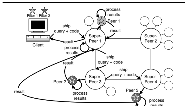
Figure 1. Pushing Code-Carrying Query Plans
