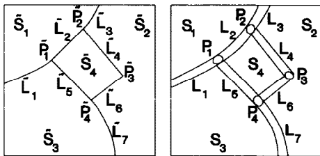
Figure 2: The image segmentation procedure: increasingly more scene knowledge is integrated into the segmentation procedure via the image model. The hypotheses generation and estimation step may be iterated for reaching more complex groupings.
