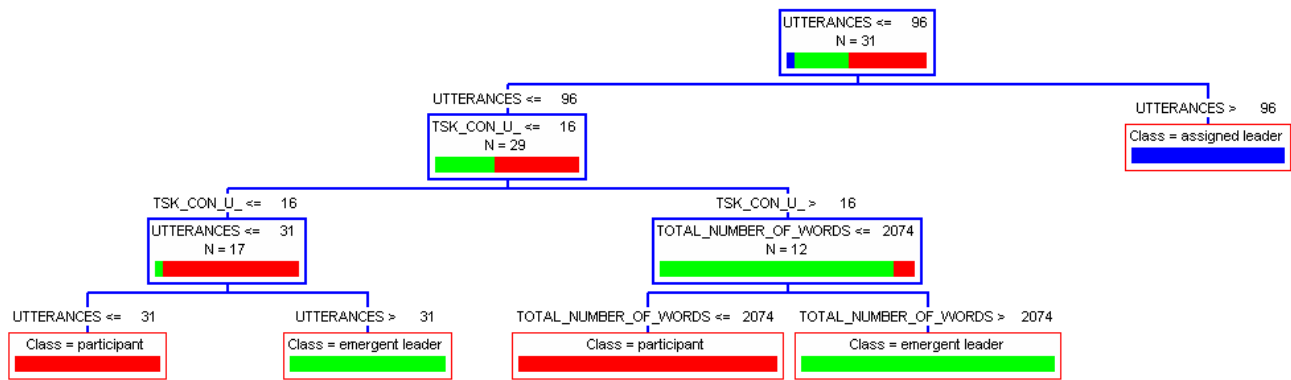
Figure 3. The decision (classification) tree for participant type in Case Study 1.
