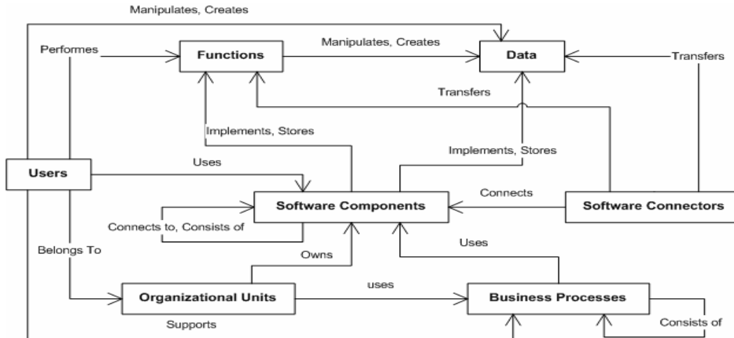
Figure 3. A basic ESSA meta-model. (Information carriers are not included in the figure since they would only make the figure more complex and their relationship to the other entities are simple).
