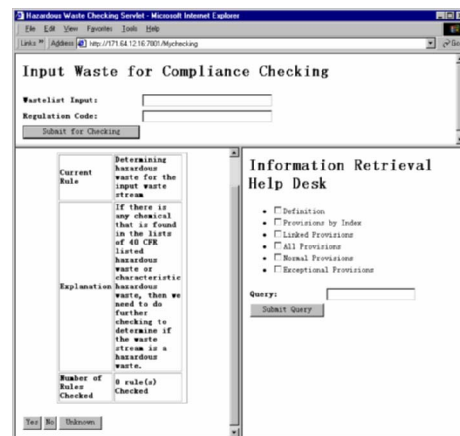
Figure 12. Web browser based user interface for hazard waste compliance checking information management system
