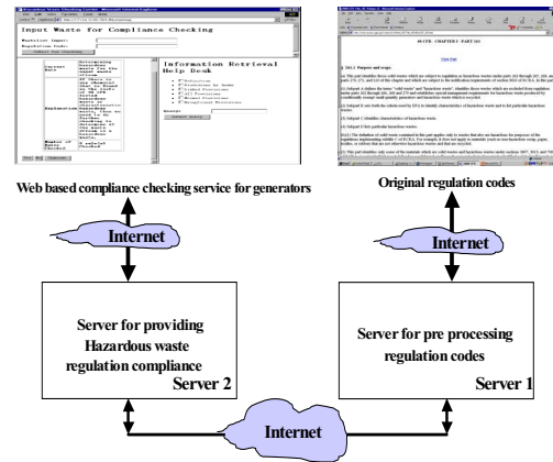
Figure 11. System architecture for the prototype system
