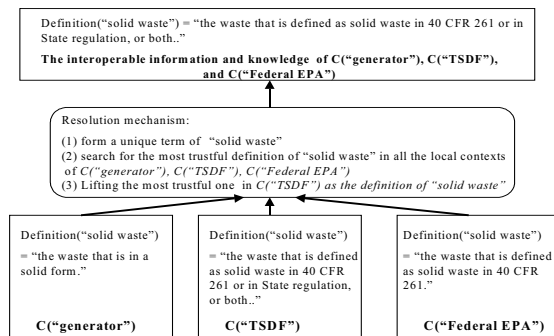
Figure 8. Using context lifting to resolve definition content conflicting from different contexts
