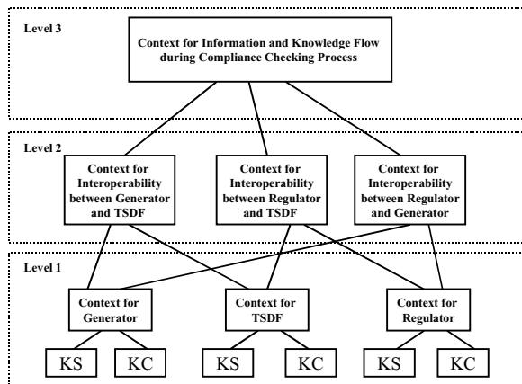
Figure 7. Hierarchy of contexts for information and knowledge flow
