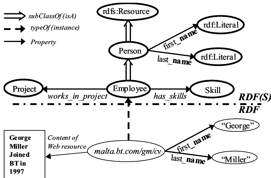
Figure 1. Ontology-based indexing.
