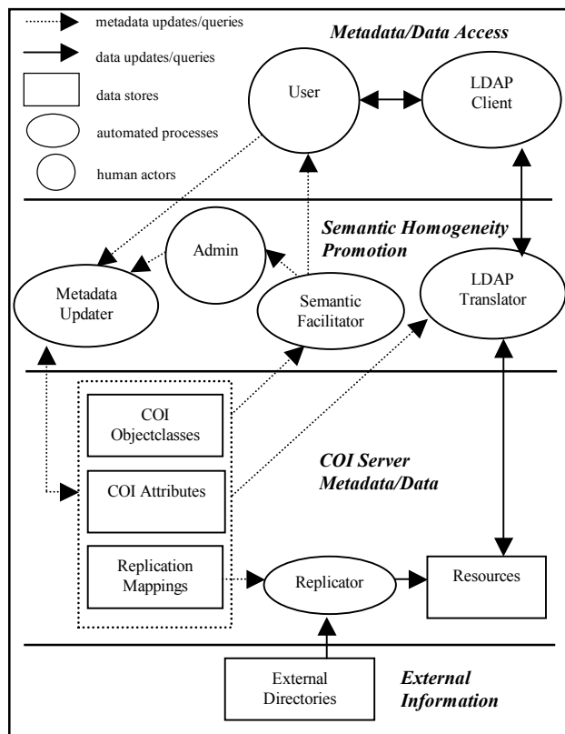
Figure 2. COI server architecture
