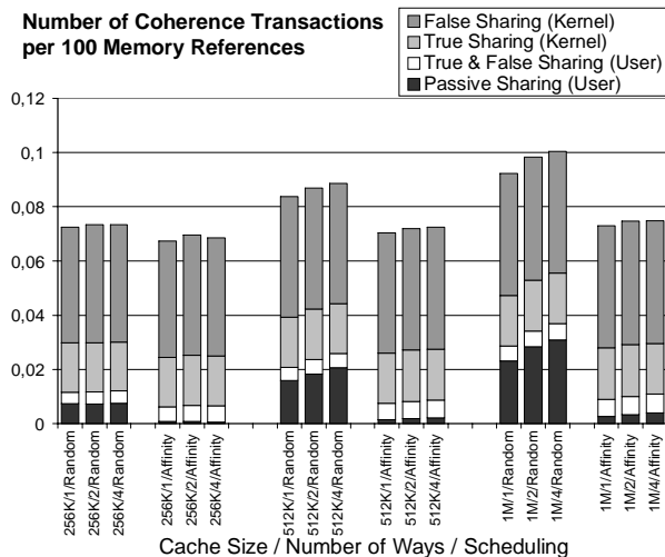
Figure 9. Number of coherence transactions ( read-and-invalidate-of-0-bytes transactions ) versus cache size (256K bytes, 512K bytes, 1M bytes), number of ways (1, 2, 4) and scheduling algorithm (random, affinity). Data assume 4 processors. Cache affinity reduces mainly passive sharing transactions; this reduction is more effective for larger cache sizes.
