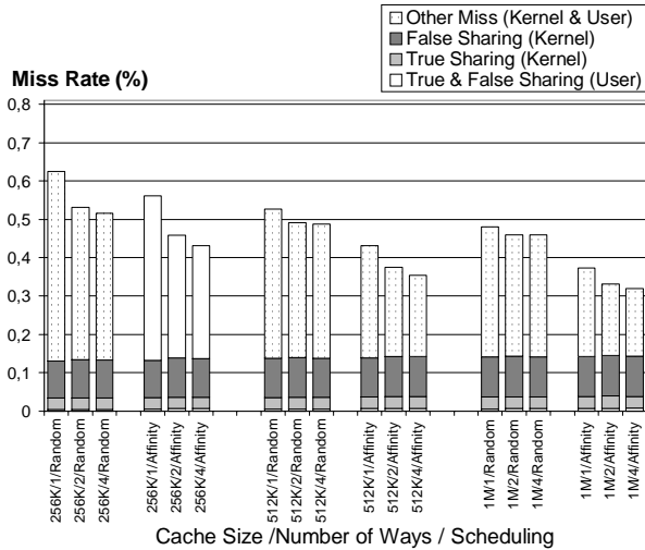
Figure 5. Breakdown of miss rate versus cache sizes (256K bytes, 512K bytes, 1M bytes), number of ways (1, 2, 4), and scheduling policy (random, affinity), for a 4-processor configuration. In case of affinity scheduler, miss rate decrease is due to the reduction of "Other Miss".
