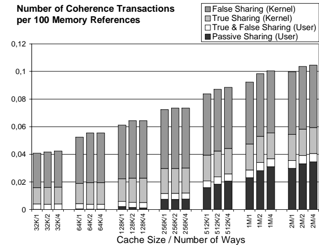
Figure 7. Number of coherence transactions ( read-and-invalidate-of-0-bytes transactions) versus cache size (32K bytes, 64K bytes, 128K bytes, 256K bytes, 512K bytes, 1M bytes, 2M bytes) and number of ways (1, 2, 4), for a 4-processor system and a random scheduling policy. Passive sharing overhead increases with large cache and higher associativity, becoming significant in case of cache sizes larger than 256K bytes
