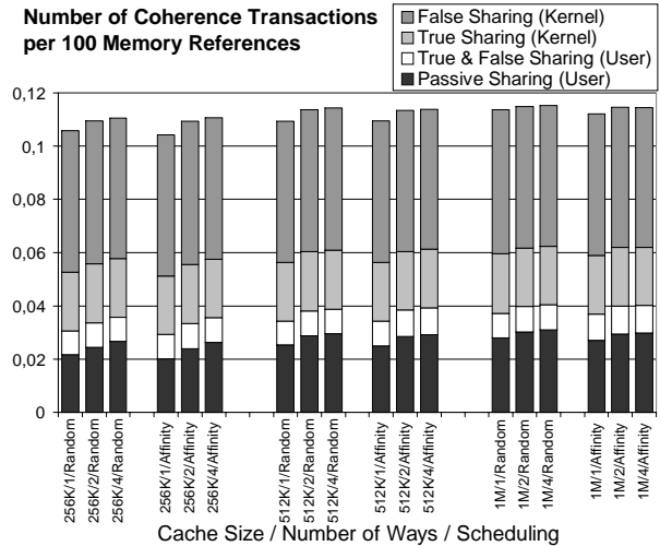
Figure 10. Number of coherence transactions ( read-and-invalidate-of-0-bytes transactions ) versus cache size (256K bytes, 512K bytes, 1M bytes), number of ways (1, 2, 4) and scheduling algorithm (random, affinity). Data assume 16 processors. In this case, affinity scheduling produces only a slightly reduction of passive sharing.
