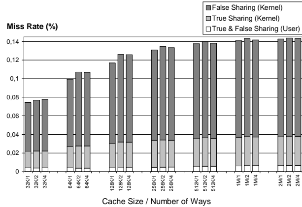
Figure 3. Breakdown of invalidation miss rate versus cache size (32K bytes, 64K bytes, 128K bytes, 256K bytes, 512K bytes, 1M bytes, 2M bytes) and number of ways (1, 2, 4), for a 4-processor system, and random scheduling policy. Invalidation misses are basically due to the kernel, and false sharing is the main source of those misses.
