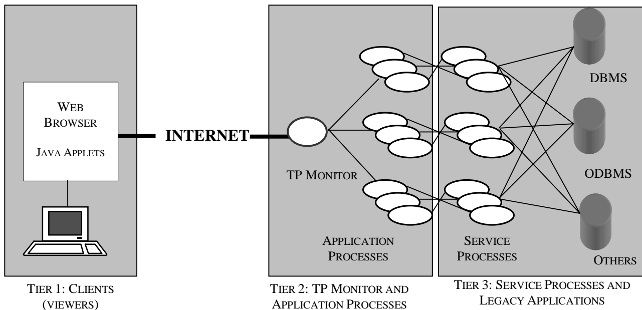
Figure 1. Typical architecture of E-Commerce application. Tier one is constituted of a client program, typically a web-browser running Java applets. Tier two is a Transaction Processing server, which includes a Transaction Processing Monitor (TP Monitor) that enables requests, spawns child application processes, and takes care of the load balance. In tier three, the service processes furnish standard services (database or other legacy applications). DBMS stands for Data Base Management System, ODBMS stands for Object-oriented Data Base Management System.
