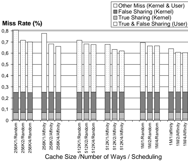
Figure 6. Breakdown of miss rate versus cache sizes (256K bytes, 512K bytes, 1M bytes), number of ways (1, 2, 4) and scheduling policy (random, affinity) for the 16-processor configuration.
