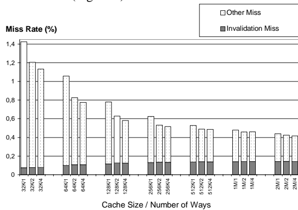
Figure 2. Breakdown of miss rate versus cache size (32K bytes, 64K bytes, 128K bytes, 256K bytes, 512K bytes, 1M bytes, 2M bytes) and number of ways (1, 2, 4), for a 4-processor system, and a random scheduling policy. "Other Miss" includes cold miss, capacity miss, and replacement miss. Miss rate decreases, whilst invalidation miss portion (i.e. the sum of false sharing misses and true sharing misses) increases with large cache size and higher associativity.
