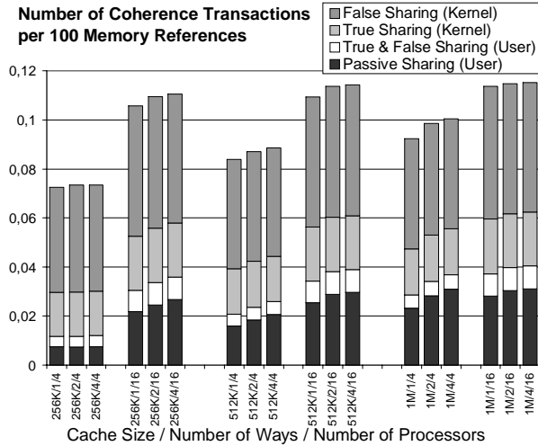
Figure 8. Number of coherence transactions ( read-and-invalidate-of-0-bytes transactions ) versus cache size (256K bytes, 512K bytes, 1M bytes), number of processors (4, 16), and number of ways (1, 2, 4), in case of a random scheduling policy. There is an increase in each component of this overhead in the “high end” (16-processor) configuration.
