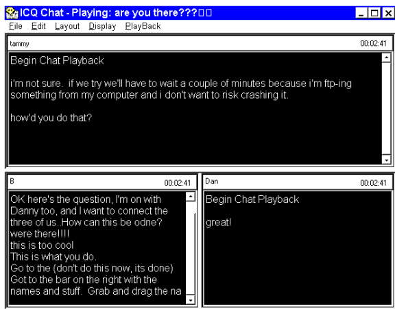
Figure 4. ICQ Chat gives each participant a window in which their words are placed, keystroke by keystroke, like UNIX Talk.
