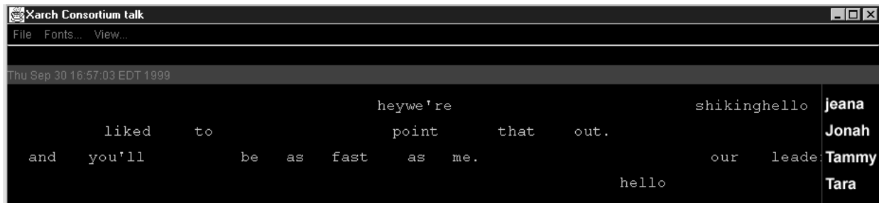
Figure 7. This is an excerpt from a four-person conversation occurring in Fugue between jeana, Jonah, Tammy and Tara. The participants are greeting and joking with each other, and commenting upon the novelty of the interface. These overlapping turns could not occur within a Chat model of conversation.
