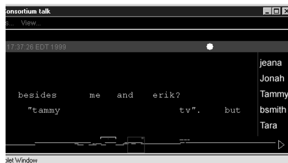
Figure 10a. The round message marker in the grey bar above the active conversation indicates that someone has added a public note to history. If it were a private note addressed to you, the round marker would have appeared within your line.
