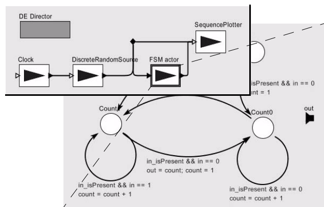
Figure 2. An FSM actor that performs run-length coding.
