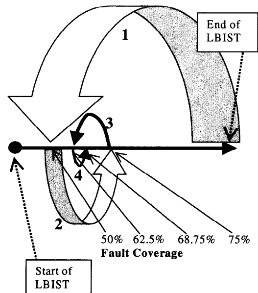
Figure 1: A binary search over fault coverage instead of patterns.
