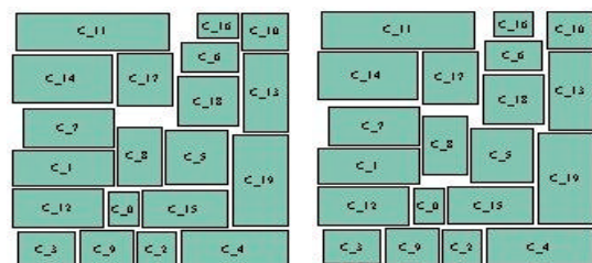
Figure 2: Minimally compacted floorplan. Left: targeted structure, right: result
