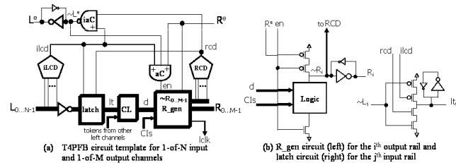
Fig. 2 T4PFB template and a detailed circuit.
