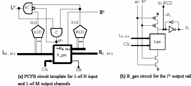
Fig. 1 PCFB template and a detailed circuit.
